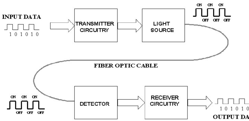
Working of Fiber optic communication
